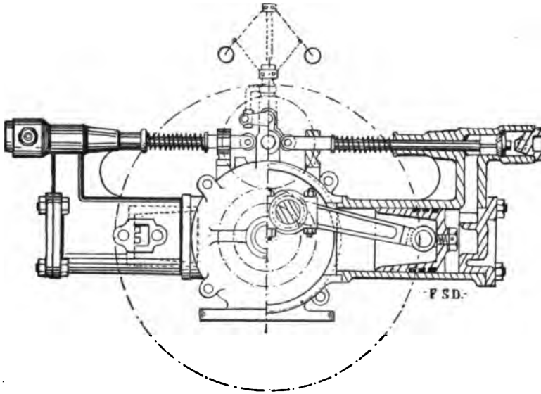
FIG. 260.—One Model of Serralte Single-acting Two-cylinder Engine. As may be seen, this engine, with cam-actuated poppet valves, centrifugal governor for regulating the cam movement, and large fly wheel, closely resembles gas engines of the double-opposed cylinder type.
